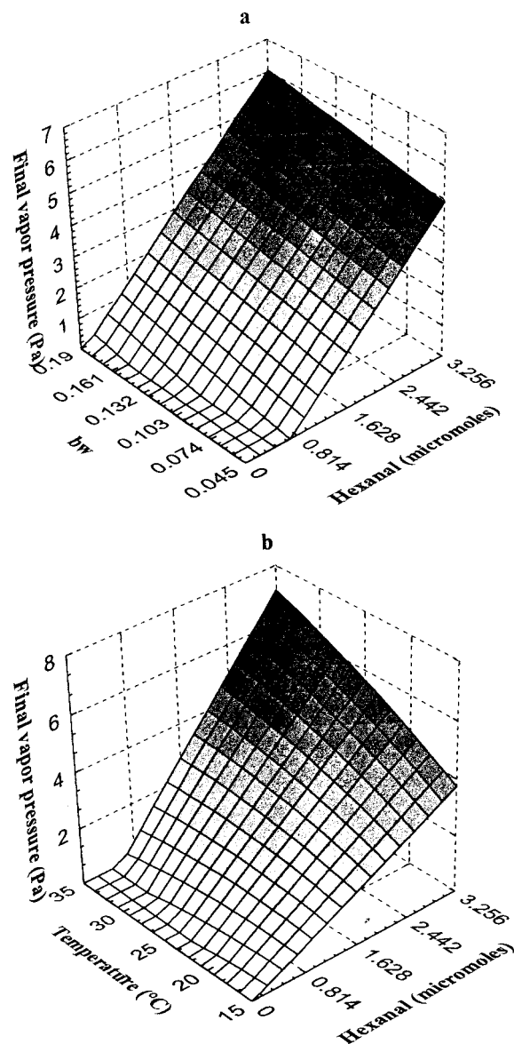
Figure 3. Three-dimensional plot relative to the interaction [b_w] \times [H] (3a), where b_w = \sqrt{1-a_w} , and to the interaction [T] \times [H] (3b) on final vapor pressure of hexanal ( P_{Hf} ).
