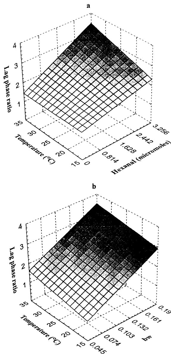
Figure 5. Three-dimensional plot relative to the interaction [H] \times [T] (5a) and to the interaction [T] \times [b_w] (5b) on lag phase ratio ( \lambda_R/\lambda_C ) for A. niger .
