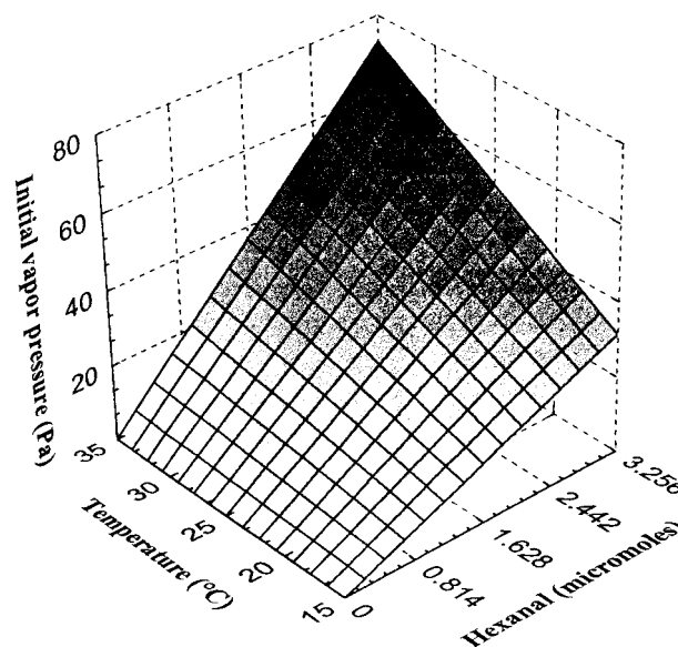
Figure 2. Three-dimensional plot relative to the interaction [T] \times [H] on initial vapor pressure of hexanal ( P_{Hi} ).
